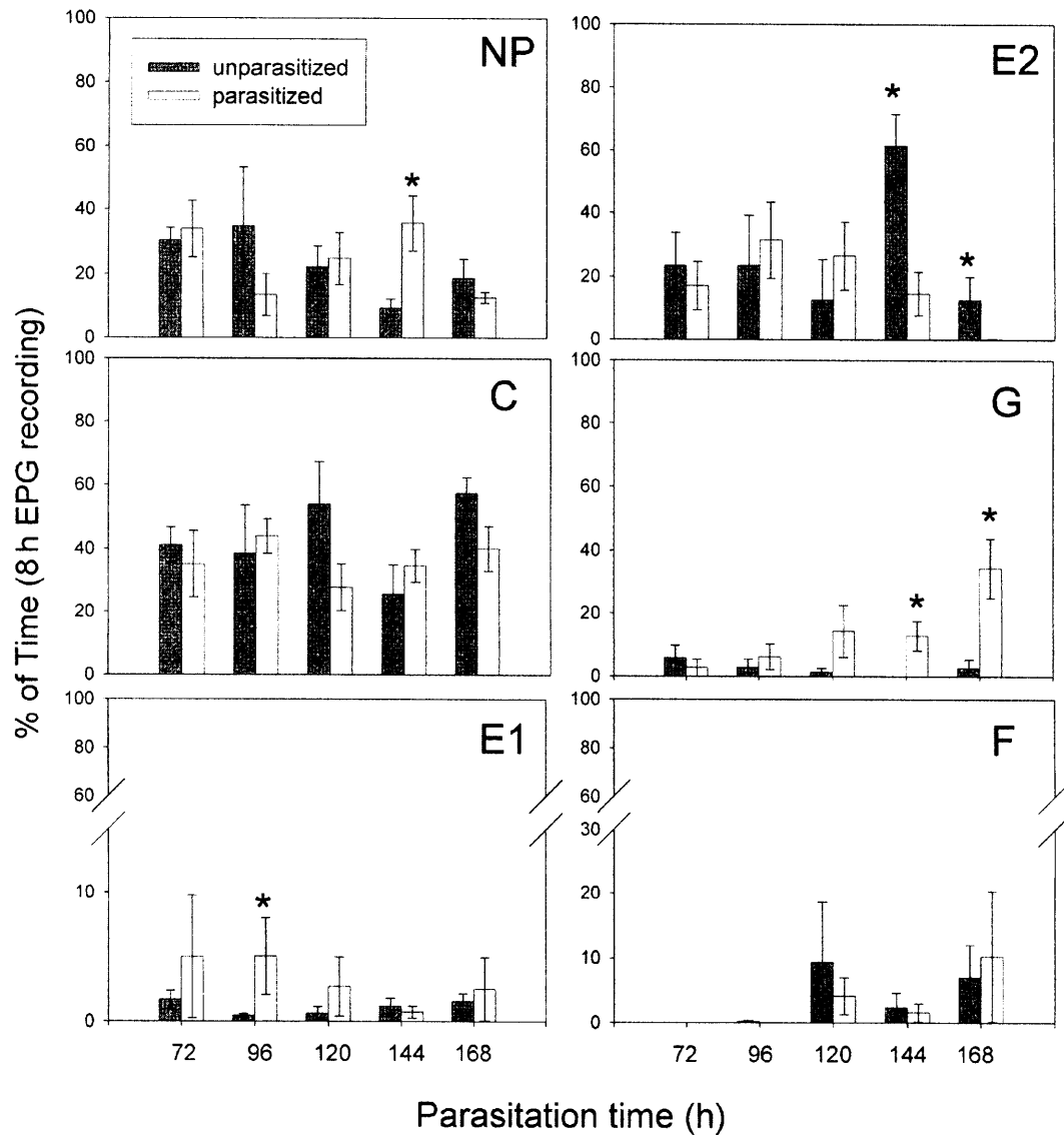
Fig. 1. Comparison of temporal changes that occurred in the times assigned to different kinds of feeding behaviour by Acyrtosiphon pisum parasitised by Aphidius ervi , relative to an unparasitised control. NP: non-penetration; C: stylet pathway phase; E1: salivation into sieve elements; E2: phloem ingestion; G: xylem ingestion; F: mechanical stylet difficulties during penetration. An asterisk indicates significant differences between treatment and control ( p < 0.05 ).
